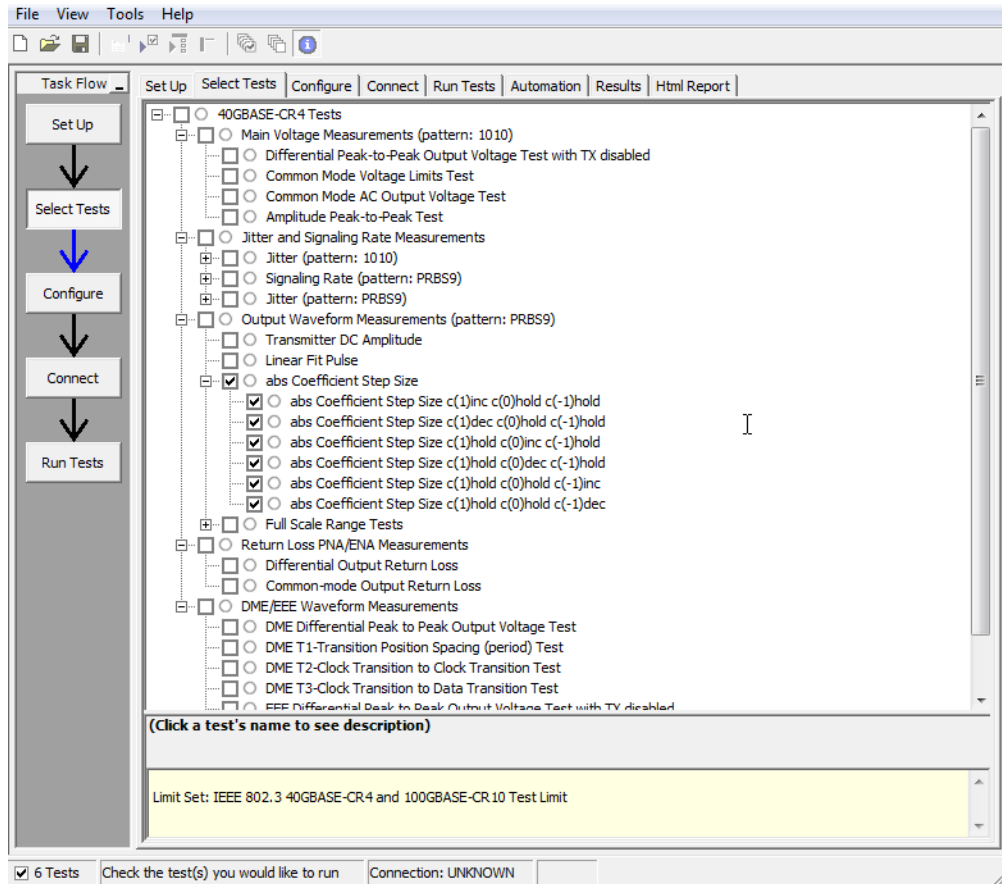
Figure 9 Selecting Transmitter Output Waveform – Abs Coefficient Step Size Test
